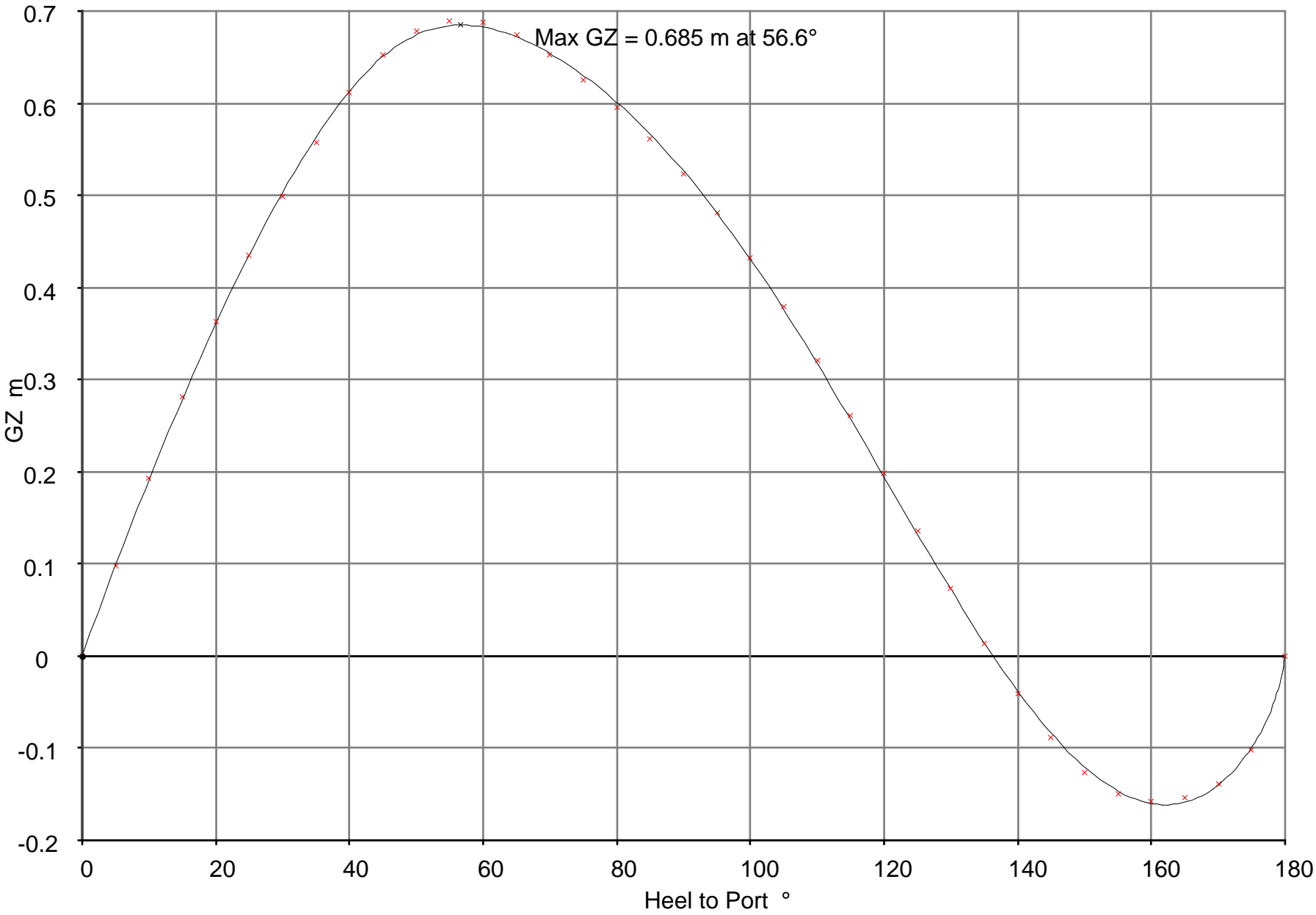
ELAN 37 GZ CURVE BASED ON IMS INCLINING AND IRC WEIGHING 20-7-04
